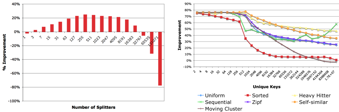
(a) Varying the number of splitters with 2^{24} unique keys. (b) Varying the number of unique keys with k = 511
