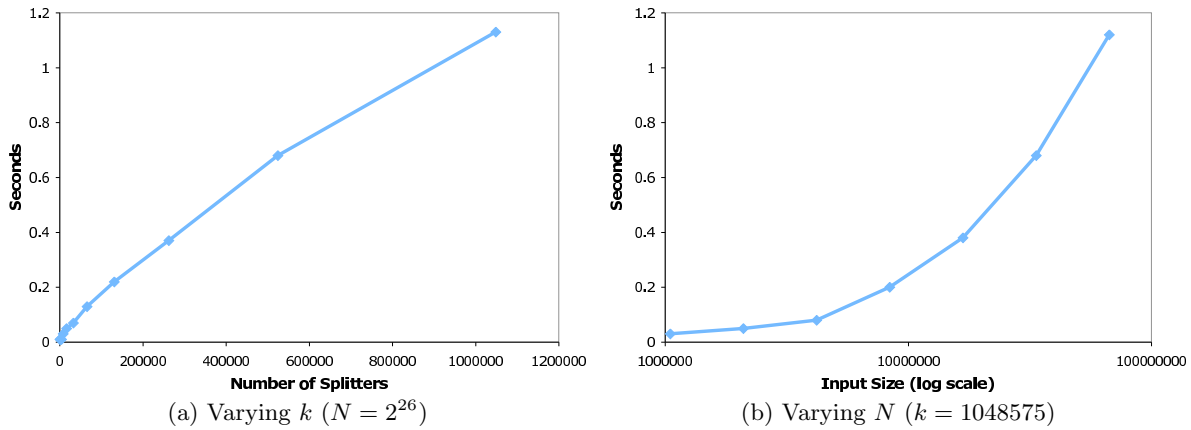
Figure 5: Time to find splitters on uniform input.
