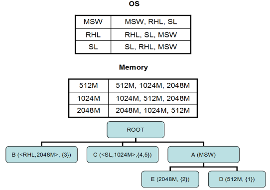
Figure 3: Similarity Lists & a Re-Ordered AL Tree.
