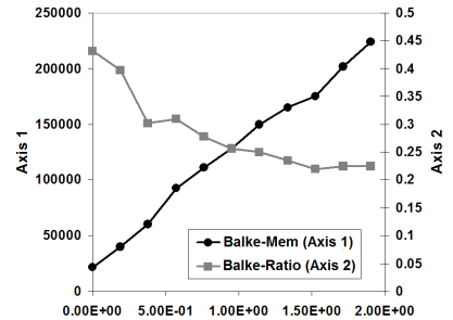
Figure 6: Balke Stats vs Density (Varying Data Size)
