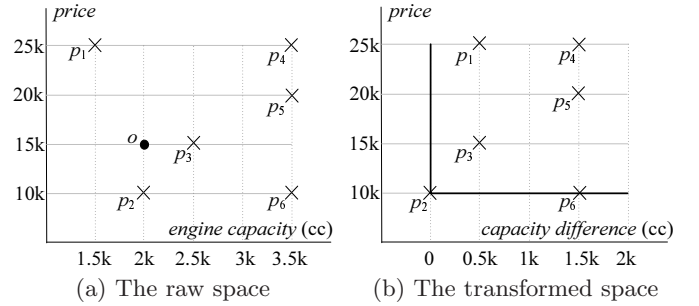
Figure 8: A dynamic skyline with bi- and uni-directional dimensions
