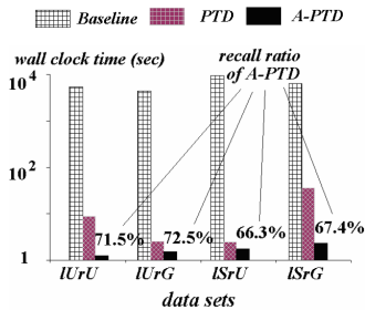
Figure 15: A-PTD Query Performance vs. Data Sets
