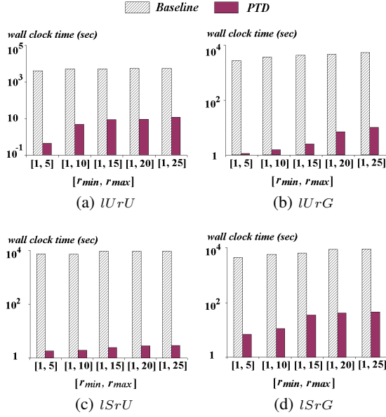
Figure 11: Performance vs. Radius Range [r_{min}, r_{max}] (Synthetic Data)
