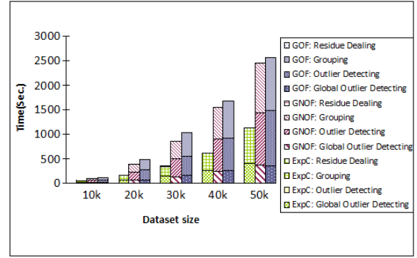
Figure 9: Performance of Four Components of ExpC , GNOF , and GOF Approaches; p=0.8 , d=0.85 , k=15
