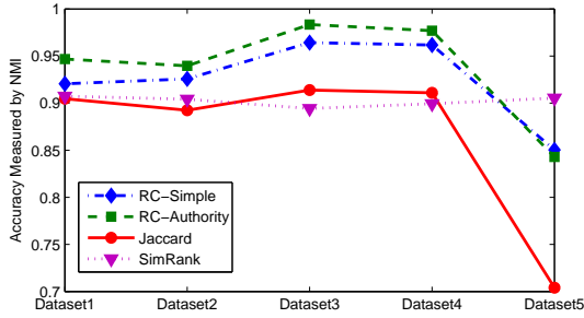
Figure 4: Accuracy of Clustering
