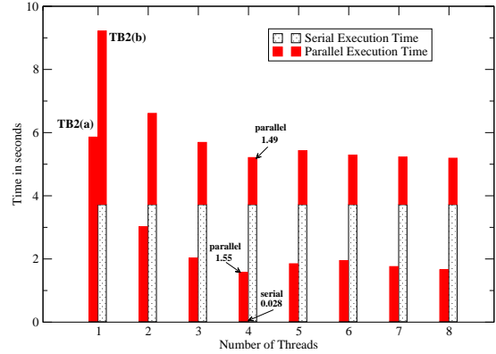
Performance of Data Partitioning on the Query TB2 Comparison of Two Data Partitioning Strategies
