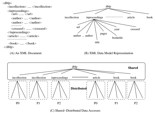
Figure 1: Partitioning an XML Document
