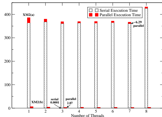
Figure 5: Data Partitioning of the query XM2. The left bar in every cluster represents the results for the XM2(A) approach, the right bar represents the results for the XML2(B) approach. In XM2(A), the overall performance is affected by the serial execution costs.
