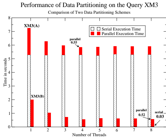
Figure 6: Data Partitioning of the query XM3 for two different queries: XM3(A), and XM3(B). The serial execution costs of the query XM3(B) are significantly lower than that of XM3(A).
