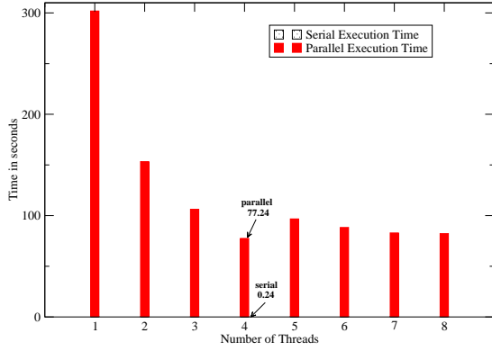
Figure 12: Data partitioning of the query DB3. The overall performance scales up as the number of threads is increased. The maximum absolute scaleup observed is 3.89 for 4 threads.
