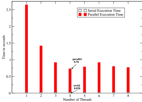
Figure 13: Data partitioning of the query TB1. The overall performance scales up as the number of threads is increased. The maximum absolute scaleup observed is 3.61 for 4 threads.
