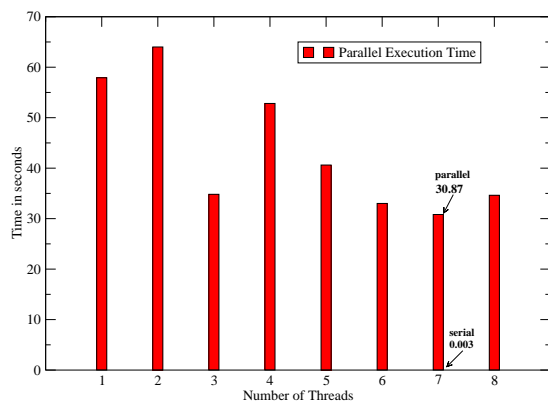
Figure 4: Data Partitioning of the query XM1. The sub-query /site/* is executed serially and the sub-query self::**/*[name(.).] is executed in parallel. The serial execution cost is too small to be represented.
