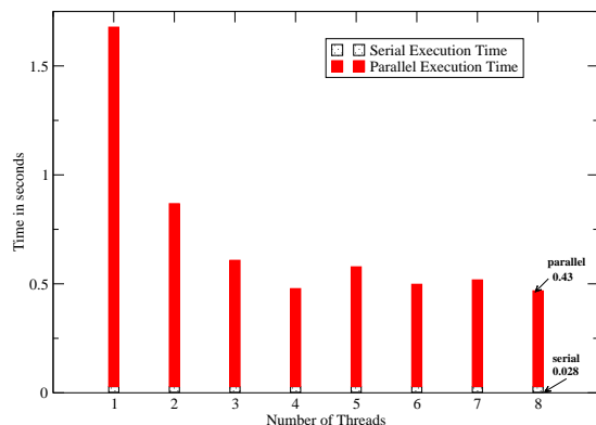
Figure 15: Data partitioning of the query TB3. Even though the performance scales up (3.89) for 8 threads, the modified query runs slower than the original query.
