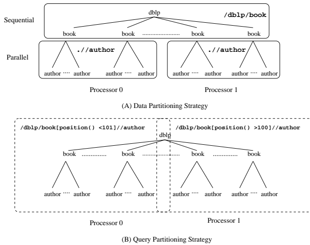
Figure 2: Parallelization of /dblp/book//author via (A) Data partitioning and (B) Query partitioning.
