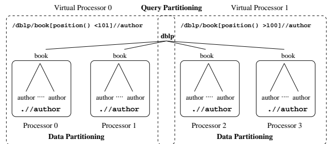
Figure 3: Parallelization of /dblp/book/author via Hybrid partitioning.
