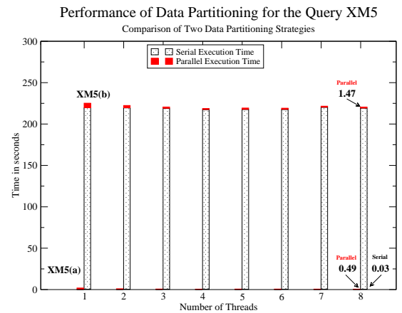
Figure 8: Data Partitioning of the query XM5 using two different partitioning strategies. XM5(B) suffers from large serial component.
