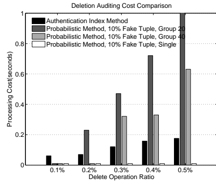
Figure 9: Deletion auditing cost
